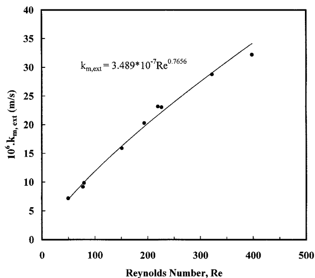
Figure 2. Measurement of external mass-transfer coefficient, k_{m,ext} , with Reynolds number.
