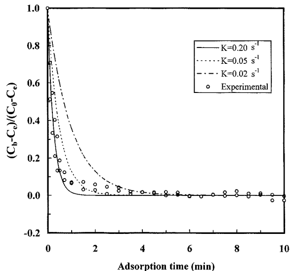
Figure 4. Determination of adsorption rate constant, K .
